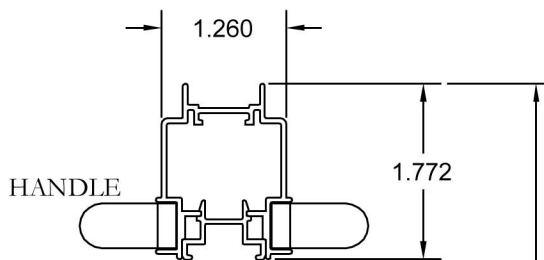
SLIDING BAR
